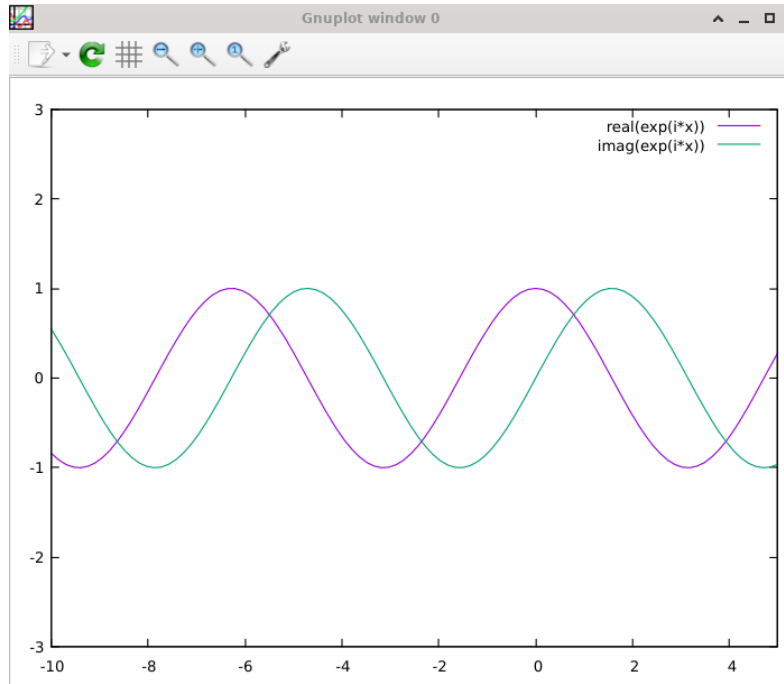
Figure 11.3: The 2D plot of the real part of e^{ix} and the imaginary part of e^{ix} (DFSimulatorC/Source Codes/C++/C++ Gnuplot SymbolicC++/ch23-Numerical Linear Algebra/2D Plot Complex Function/main.cpp).
