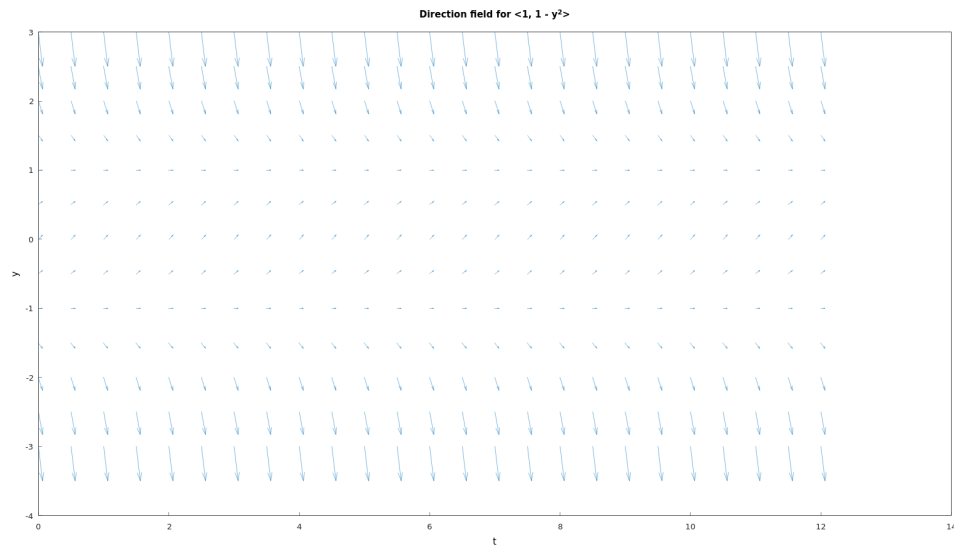
Figure 4.48: The direction field for \frac{dy}{dt} = 1 - y^2 . Solution curves in the ty -plane corresponding to \alpha = 1 are tangent to the vectors in the direction field \langle 1, 1 - y^2 \rangle at every point (Hamzstplot/Examples with Makefile/Differential Equations/Plot Direction Fields for Bifurcation Points Problem 25c/main.cpp).
