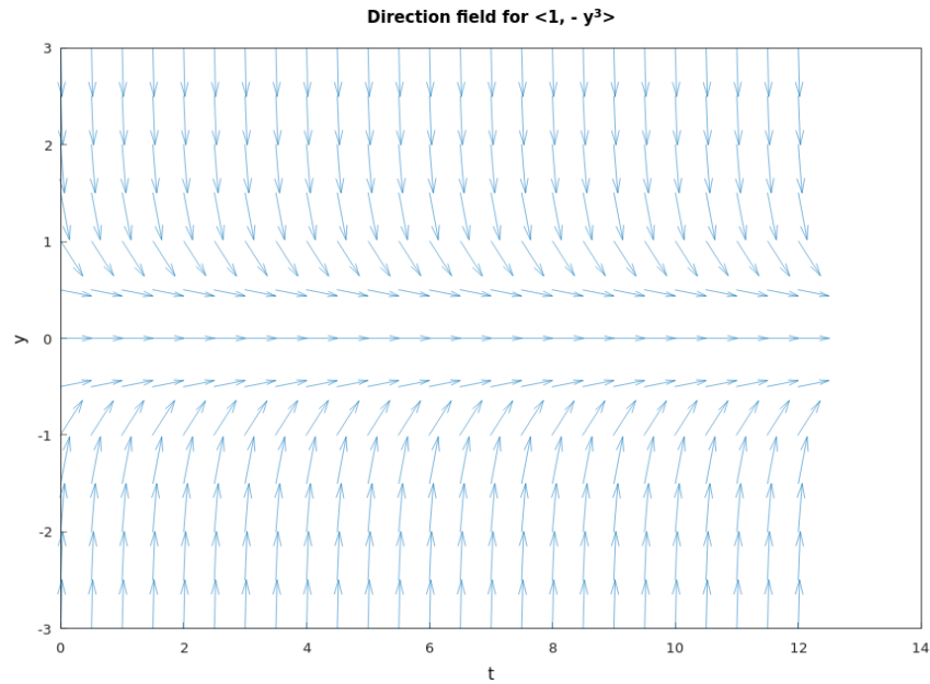
Figure 4.54: The direction field for \frac{dy}{dt} = -y^3 . Solution curves in the ty -plane corresponding to \alpha = 0 are tangent to the vectors in the direction field \langle 1, -y^3 \rangle at every point (Hamzstplot/Examples with Makefile/Differential Equations/Plot Direction Fields for Bifurcation Points Problem 26b/main.cpp).
