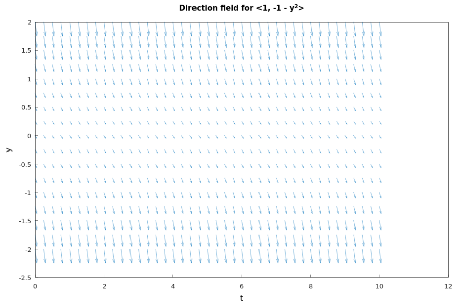
Figure 4.46: The direction field for \frac{dy}{dt} = -1 - y^2 . Solution curves in the ty -plane corresponding to \alpha = -1 are tangent to the vectors in the direction field \langle 1, -1 - y^2 \rangle at every point ( Hamzstplot/Examples with Makefile/Differential Equations/Plot Direction Fields for Bifurcation Points Problem 25a/main.cpp ).
