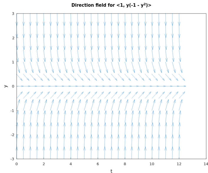
Figure 4.53: The direction field for \frac{dy}{dt} = y(-1 - y^2) . Solution curves in the ty -plane corresponding to \alpha = 1 are tangent to the vectors in the direction field \langle 1, y(-1 - y^2) \rangle at every point (Hamzstplot/Examples with Makefile/Differential Equations/Plot Direction Fields for Bifurcation Points Problem 26a/main.cpp).
