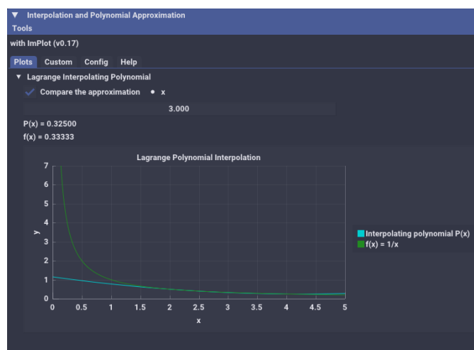
Figure 10.7: The plot for Lagrange interpolating polynomial with Hamzstlab, SymIntegration and Armadillo for f(x) = \frac{1}{x} with nodes x_0 = 2, x_1 = 2.5 , and x_2 = 4 . (Hamzstlab-Mathematics/examples/Interpolation/main.cpp).
