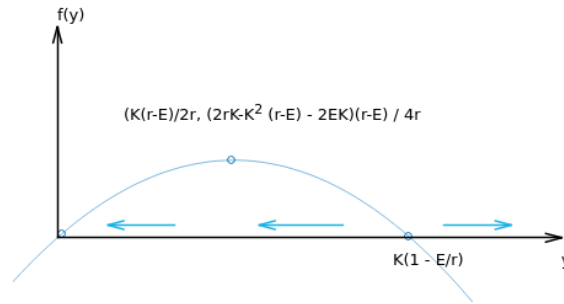
Figure 4.37: The equilibrium points and the stability analysis for \frac{dy}{dt} = f(y) = \left(y - K\left(1 - \frac{E}{r}\right)\right)y (Hamzstplot/Examples with Makefile/Differential Equations/Plot 2D Equilibrium Solution for Schaefer Modell/main.cpp).
