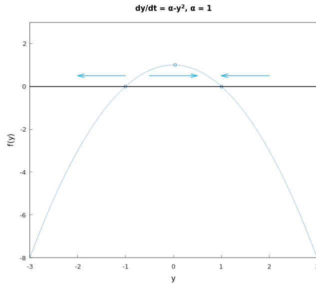
Figure 4.45: The plot for f(y) = \alpha - y^2 with \alpha = 1 , the phase line is drawn with the blue arrows ( Hamzstplot/Examples with Makefile/Differential Equations/Plot 2D for Bifurcation Points Problem 25 2 Equilibrium Solutions/main.cpp ).
