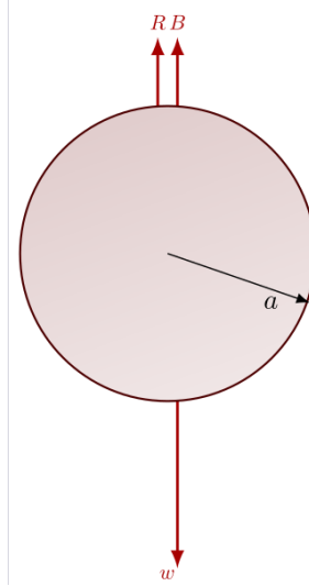
Figure 4.14: The free-body diagram for a sphere shape body falling in a dense fluid.
