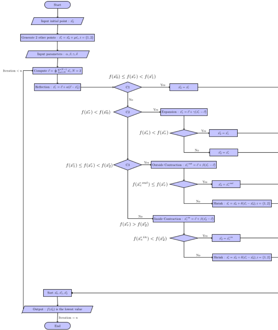
Figure 10.19: The flowchart for downhill simplex algorithm that is used to make the C++ code for computing the solution.
