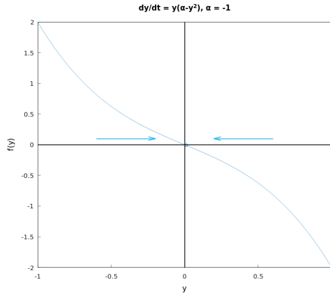
Figure 4.50: The plot for f(y) = y(\alpha - y^2) with \alpha = -1 , the phase line is drawn with the blue arrows ( Hamzstplot/Examples with Makefile/Differential Equations/Plot 2D for Bifurcation Points Problem 26 Only 1 Equilibrium Solution/main.cpp ).
