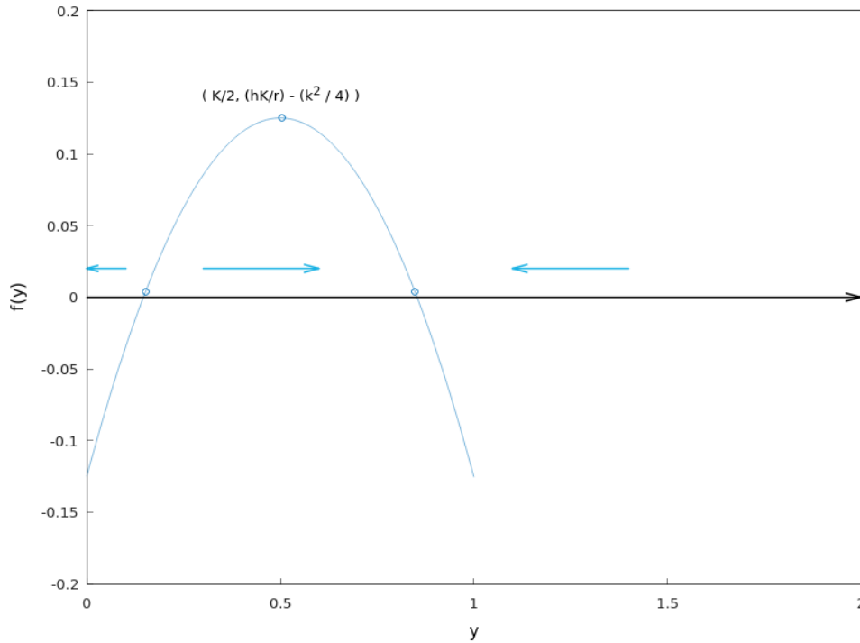
Figure 4.39: The plot for f(y) = (1 - y)y - \frac{1}{8} (Hamzstplot/Examples with Makefile/Differential Equations/Plot 2D Equilibrium Solution for Schaefer Model Variation/main.cpp).
