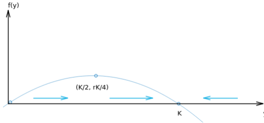
Figure 4.30: The equilibrium solution f(y) = 0 or r(1 - y/K)y = 0 to visualize other solutions of Eq. (5.59) ( Hamzstplot/Examples with Makefile/Differential Equations/Plot 2D Equilibrium Solution for Logistic Growth/main.cpp ).
