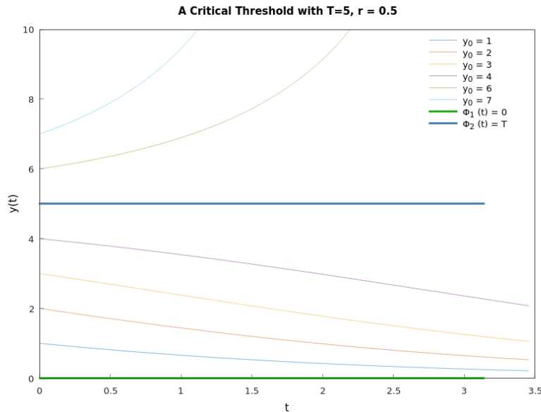
Figure 4.34: The solution curves for growth with a threshold for \frac{dy}{dt} = -r \left(1 - \frac{y}{T}\right) y (Hamzstplot/Examples with Makefile/Differential Equations/Plot 2D Solution Curves for Critical Threshold/main.cpp).
