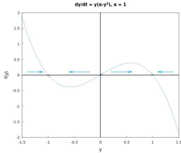
Figure 4.52: The plot for f(y) = y(\alpha - y^2) with \alpha = 1 , the phase line is drawn with the blue arrows (Hamzstplot/Examples with Makefile/Differential Equations/Plot 2D for Bifurcation Points Problem 26 2 Equilibrium Solutions/main.cpp).
