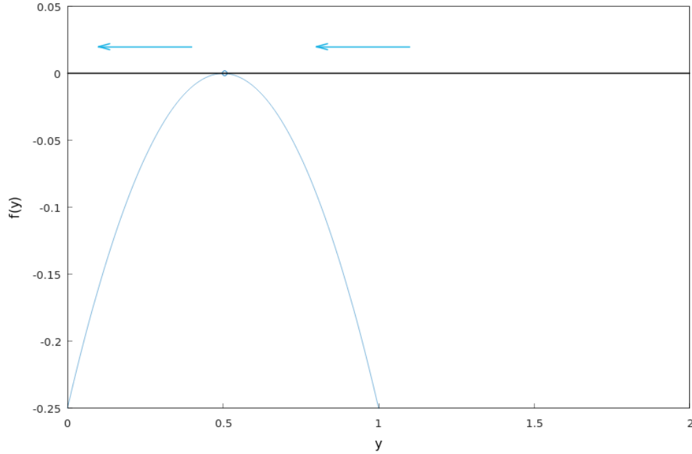
Figure 4.41: The plot for f(y) = (1-y)y - \frac{1}{4} (Hamzstplot/Examples with Makefile/Differential Equations/Plot 2D Equilibrium Solution Only 1 for Schaefer Model Variation/main.cpp).
