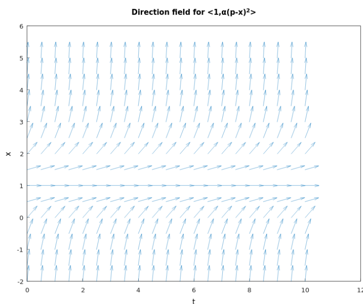
Figure 4.58: The direction field for \langle 1, \alpha(p-x)^2 \rangle with \alpha = 1 and p = 1 (Hamzstplot/Examples with Make-file/Differential Equations/Plot Direction Fields for Chemical Reactions Problem 28b/main.cpp).
