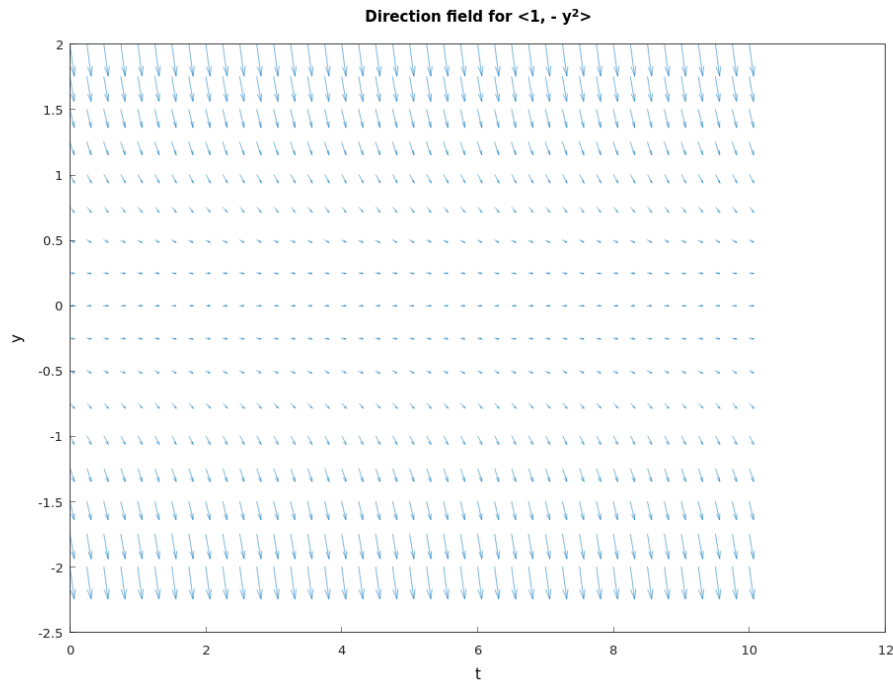
Figure 4.47: The direction field for \frac{dy}{dt} = -y^2 . Solution curves in the ty -plane corresponding to \alpha = 0 are tangent to the vectors in the direction field \langle 1, -y^2 \rangle at every point (Hamzstplot/Examples with Makefile/Differential Equations/Plot Direction Fields for Bifurcation Points Problem 25b/main.cpp).
