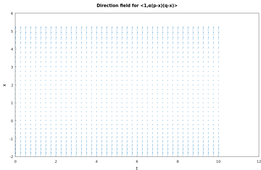
Figure 4.57: The direction field for \langle 1, \alpha(p - x)(q - x) \rangle with \alpha = 1 , p = 1 , and q = 2 (Hamzstplot/Examples with Makefile/Differential Equations/Plot Direction Fields for Chemical Reactions Problem 28a/main.cpp).
