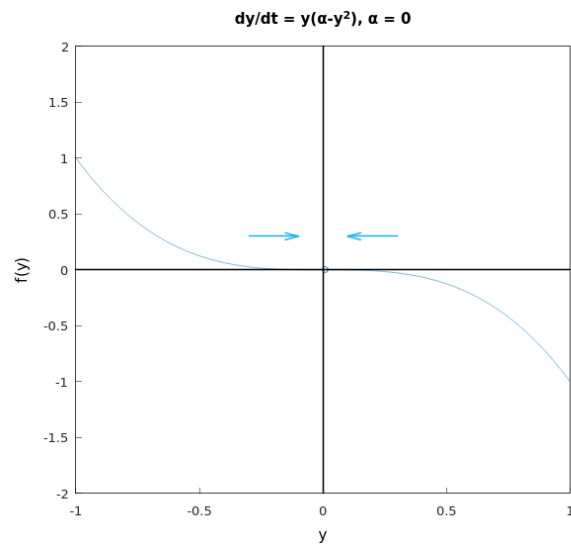
Figure 4.51: The plot for f(y) = y(\alpha - y^2) with \alpha = 0 , the phase line is drawn with the blue arrows ( Hamzstplot/Examples with Makefile/Differential Equations/Plot 2D for Bifurcation Points Problem 26 Only 1 Equilibrium Solution/main.cpp ).
