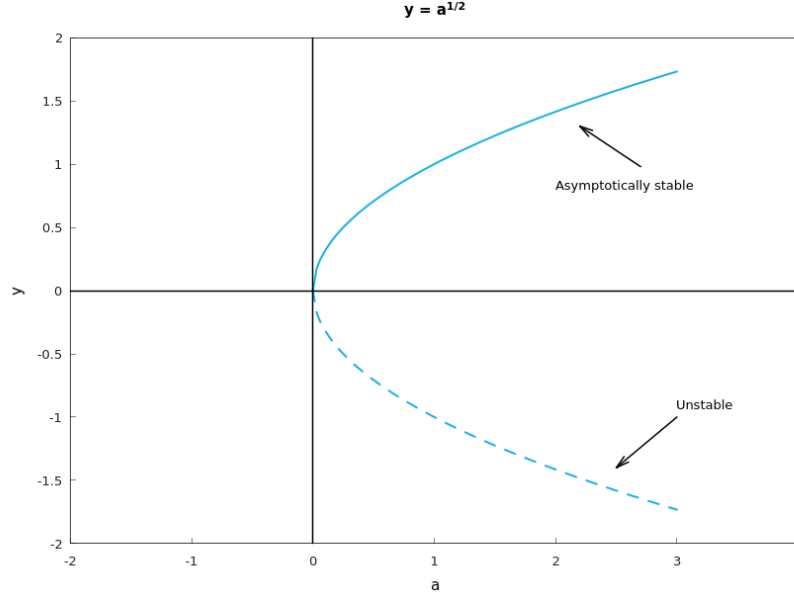
Figure 4.49: The bifurcation diagram for \frac{dy}{dt} = a - y^2 , the bifurcation point at a = 0 is called a saddle-node bifurcation where the solution then differ into two kind of solution: stable and unstable (Hamzstplot/Examples with Makefile/Differential Equations/Plot 2D Bifurcation Diagram Problem 25/main.cpp).
