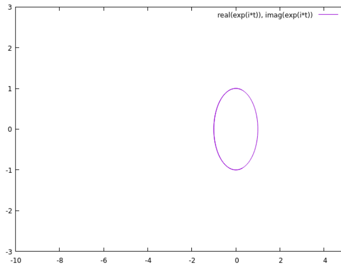
Figure 11.4: The 2D parametric plot of (\text{real}(e^{ix}), \text{imag}(e^{ix})) (DFSimulatorC/Source Codes/C++/C++ Gnuplot SymbolicC++/ch23-Numerical Linear Algebra/2D Plot Complex Function/main.cpp).
