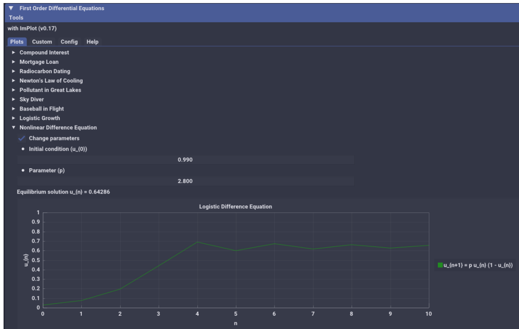
Figure 4.68: The interactive plot for solutions of nonlinear difference equation for the logistic difference equation at Eq. (5.147) with varying \rho and initial conditions u_0 with Hamzstlab Mathematics. (Hamzstlab-Mathematics/examples/First Order Differential Equation/main.cpp).
