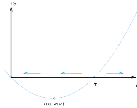
Figure 4.33: The graph of f(y) for \frac{dy}{dt} = -r \left(1 - \frac{y}{T}\right) y (Hamzstplot/Examples with Makefile/Differential Equations/Plot 2D Equilibrium Solution for Critical Threshold/main.cpp).
